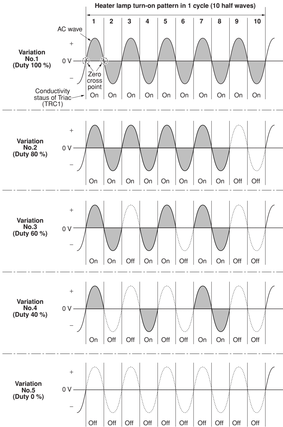
Figure 2-3-7 Heater lamp turn-on variations
