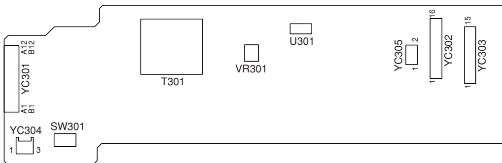
Figure 2-3-12 Bias board silk-screen diagram
