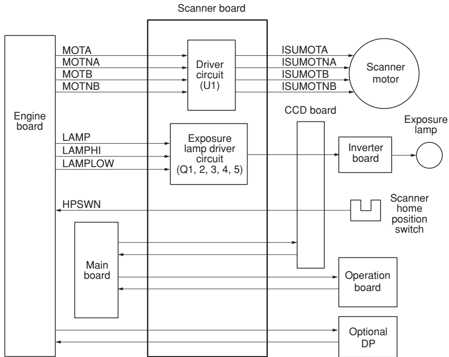
Figure 2-3-20 Scanner board circuit block diagram
